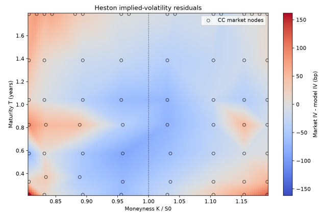
(b) Heston
